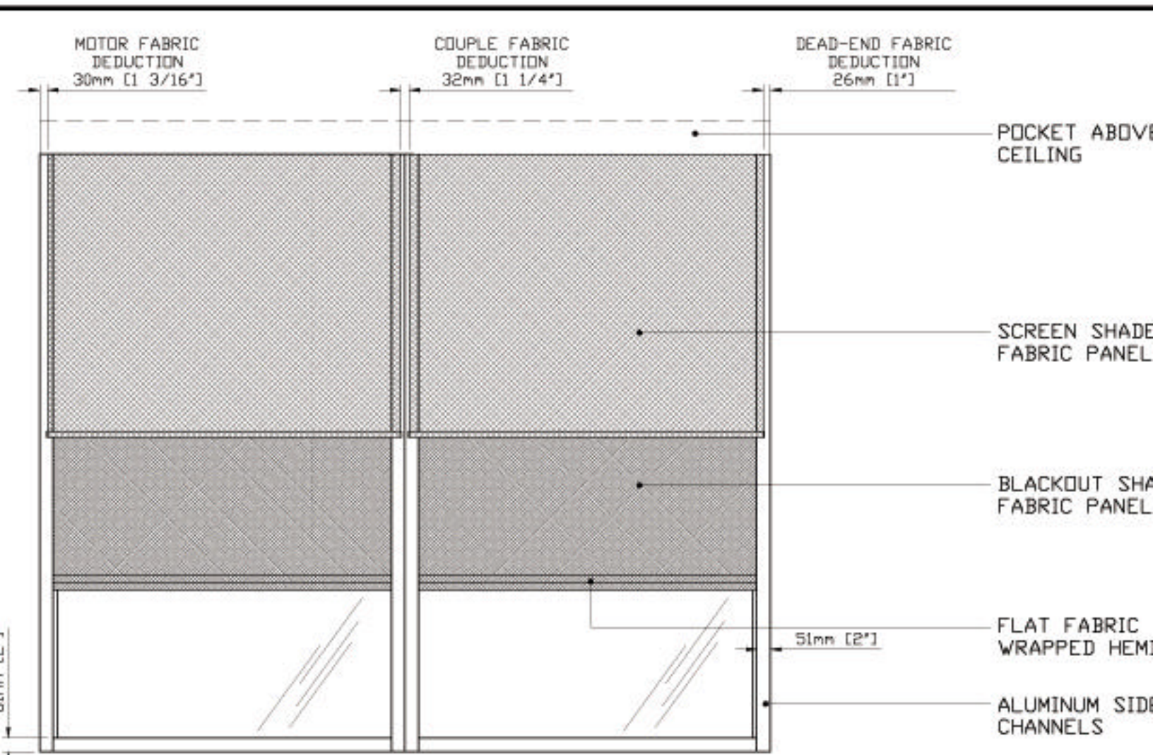
1 DUAL MOTOR SHADE IN A POCKET NTS
