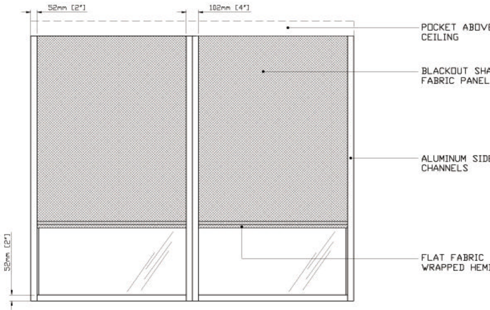
1 BLACKOUT MOTOR SHADE IN A POCKET NTS
